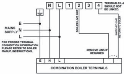
1. Typical combination boiler installation
