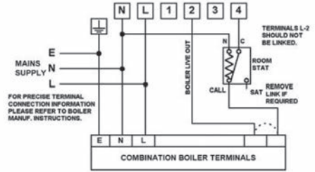
2. Typical combination boiler installation with Room Stat
